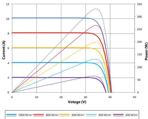
Current-Voltage & Power-Voltage Curve (330S)
